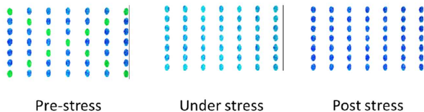
Fig. 2.6: A 7 \times 7 array corresponding to the black segment of an image with randomly corrupted pixels (black pixels turned white). Application and subsequent removal of global stress applied along the major axes of the elliptical nanomagnets corrects the corrupted pixels and turns them all black.
