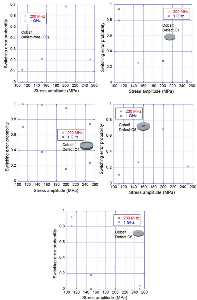
Fig. 3.13: Switching error probability at room temperature as a function of applied uniaxial stress amplitude of a surface acoustic wave of frequency 200 MHz and 1 GHz for a cobalt elliptical nanomagnet of nominal major axis 100 nm, minor axis 90 nm and thickness 6 nm. The plots are for the defect-free and defective nanomagnets with defects C1, C4, C5 and C6.
