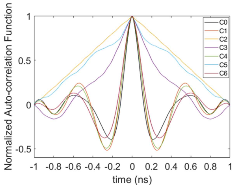
Fig. 5.2: The normalized temporal auto-correlation functions (defined in Equation (1)) plotted as a function of time for defect-free and defective LBMs. All LBMs in this plot are nominally identical, except they have different defects. Their auto-correlation functions are very different – both qualitatively and quantitatively – showing that this parameter is unpredictable in real LBMs that have random defects. Single (C1 and C4), and multiple (C6) localized defects do not change the auto-correlation functions by much, but delocalized (extended) defects (C2, C3 and C5) affect the auto-correlation functions drastically.
