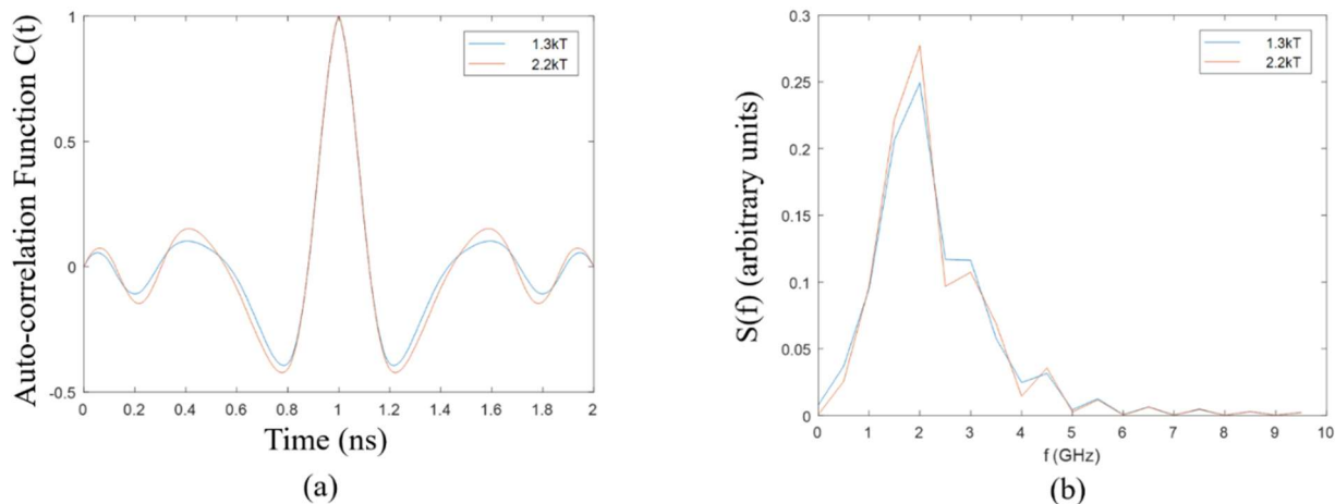
Fig. 5.5: (a) Normalized auto-correlation functions of two LBMs with energy barriers of 1.3 kT and 2.2 kT, (b) Power spectral densities of two LBMs with energy barriers of 1.3 kT and 2.2 kT.
