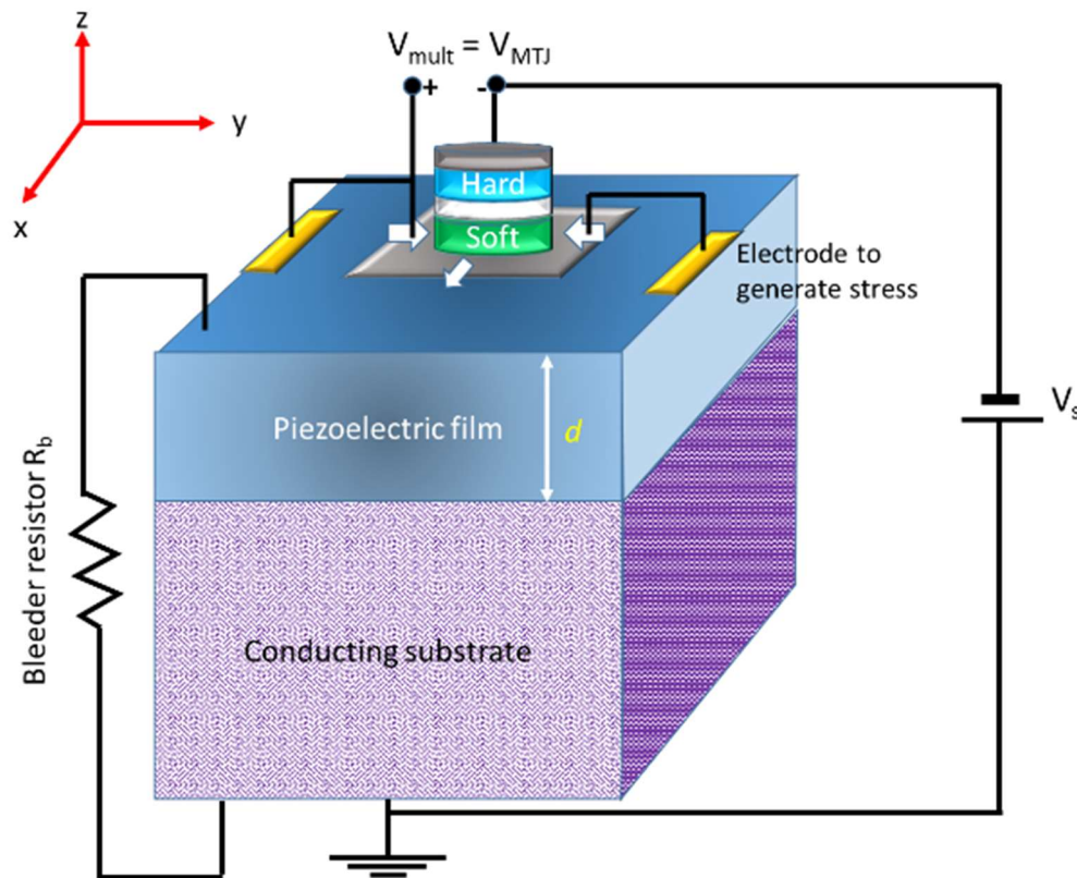
Fig. 6.1: A microwave oscillator implemented with a single straintronic magneto-tunneling junction (MTJ) and a passive resistor. The output voltage of the device is V_{mult} which is the voltage dropped over the MTJ. The strain generated in the elliptical MTJ soft layer due to the voltage dropped over the piezoelectric is biaxial (compressive along the major axis and tensile along the minor axis). The white arrows show the strain directions. The piezoelectric layer is poled in the vertically up direction. The lateral dimension of the soft layer, the spacing between the edge of the soft layer and the nearest electrode, and the piezoelectric film thickness are all approximately the same and that generates biaxial strain in the soft layer [23].
